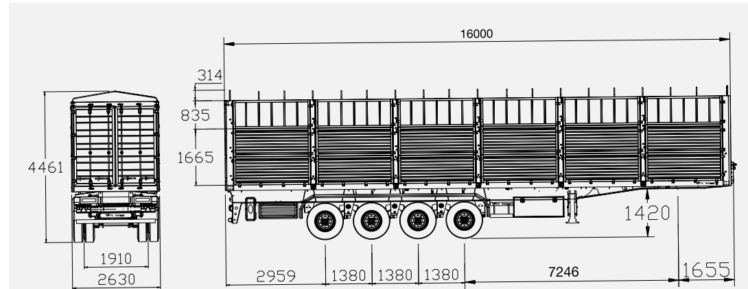
MECHANICAL SUSPENSION 4 X 14 T AXLE TIRES 12 R 22,5 - 16+1 PCS
